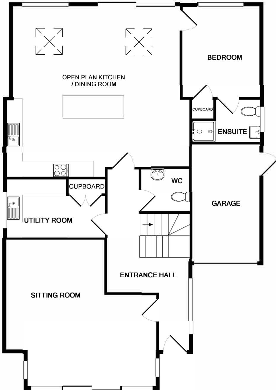
GROUND FLOOR APPROX. FLOOR AREA 128.9 SQ.M. (1388 SQ.FT.)
