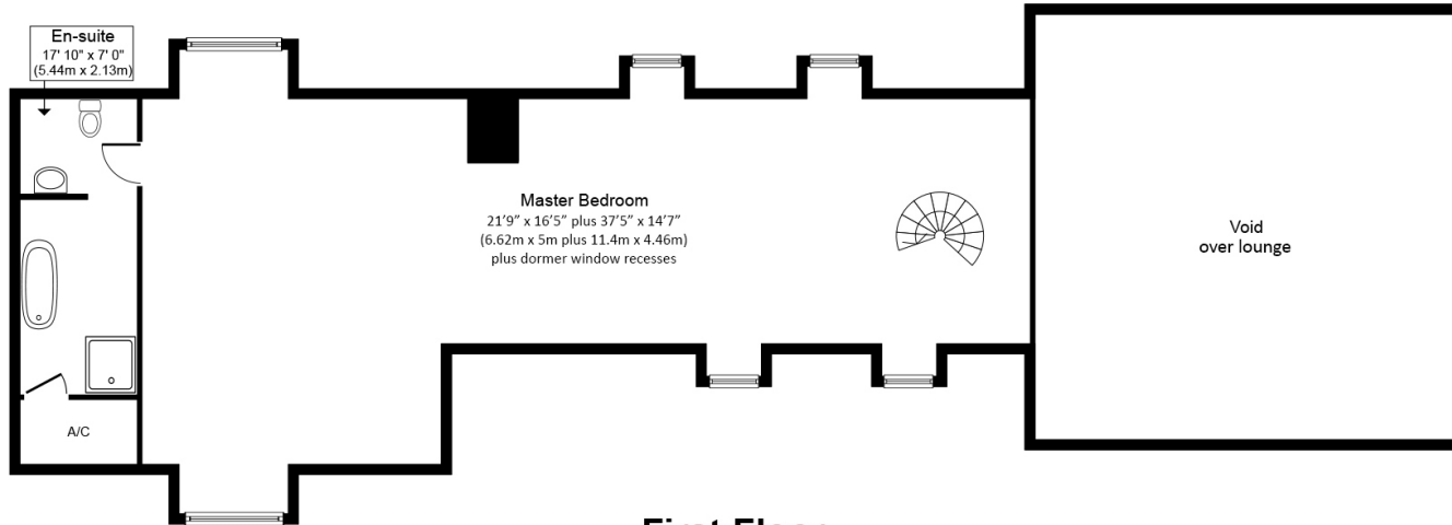
First Floor Approximate Floor Area 1,130 sq. ft (105.5 sq.m)
