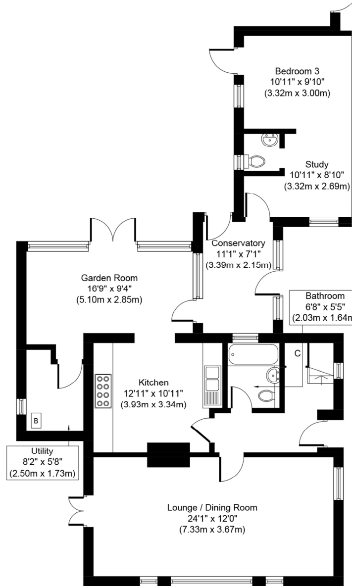
Ground Floor Approximate Floor Area 1063 Sq. ft. (98.8 Sq. m.)
