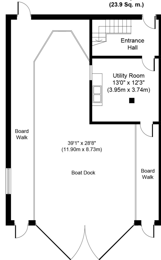
Boat House - Ground Floor Approximate Floor Area 257 Sq. ft. (23.9 Sq. m.)
