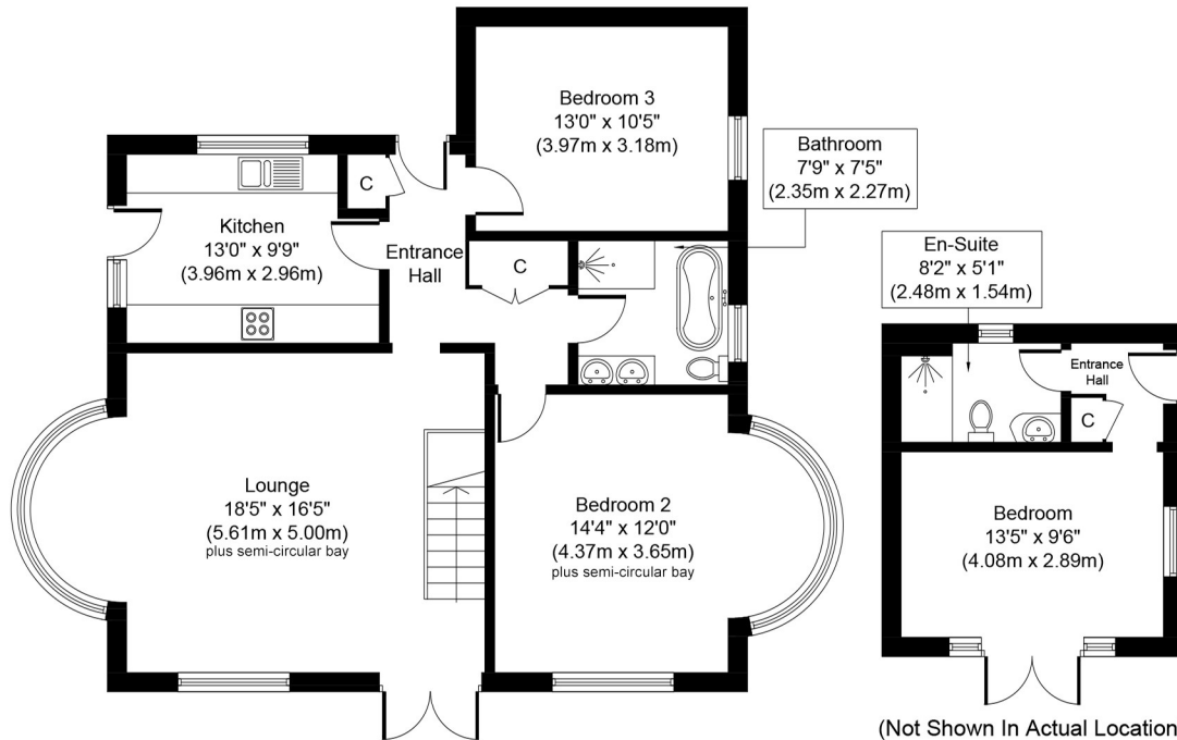
Ground Floor Approximate Floor Area 978 Sq. ft. (90.9 Sq. m.)
