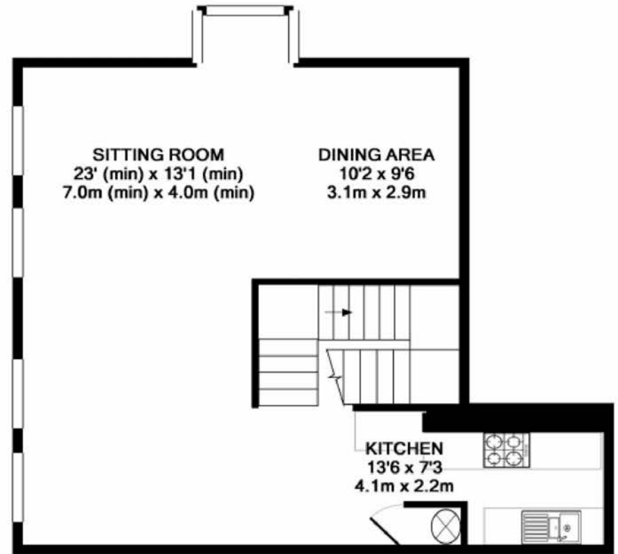
1ST FLOOR APPROX. FLOOR AREA 572 SQ.FT. (53.2 SQ.M.)
