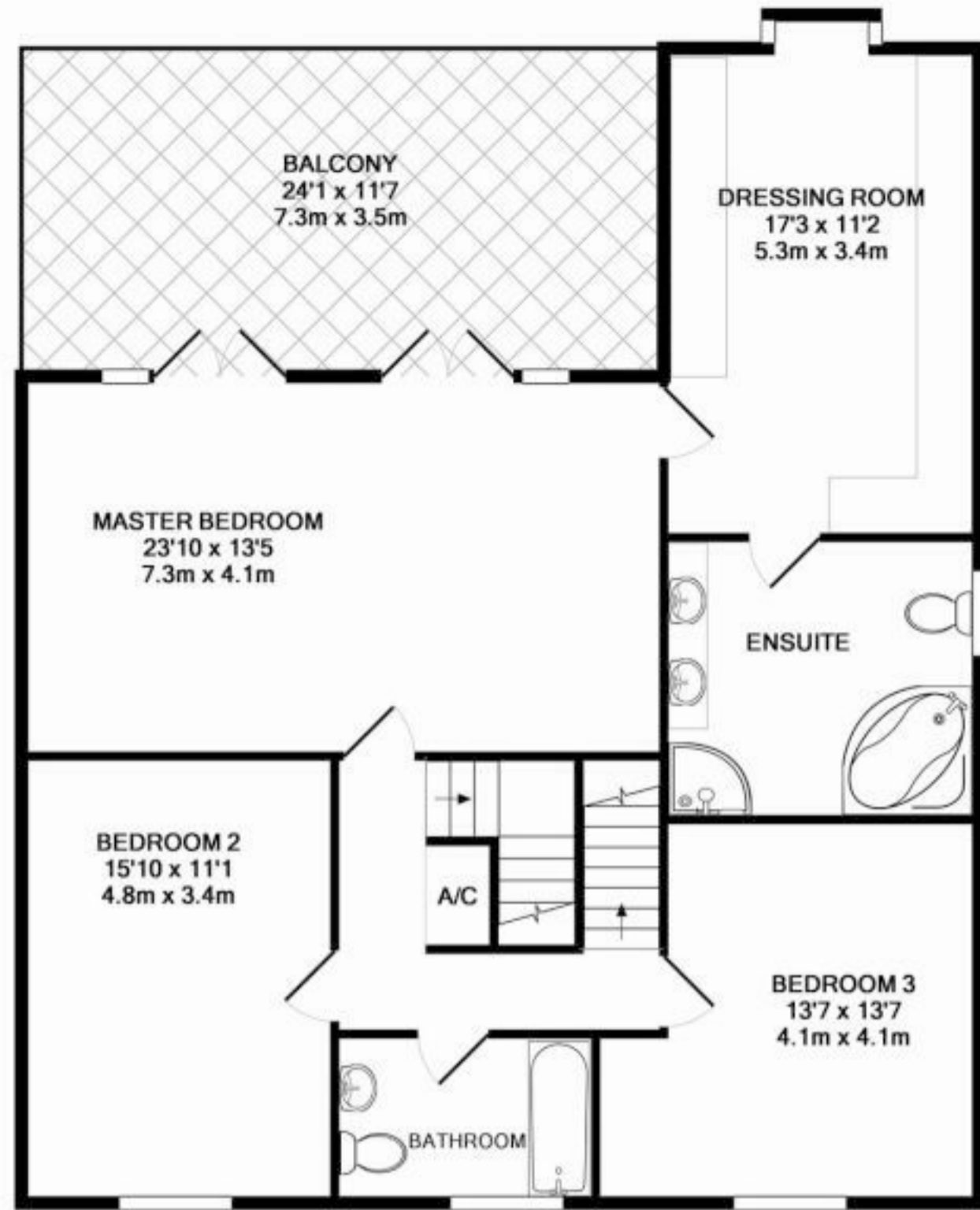
1ST FLOOR
