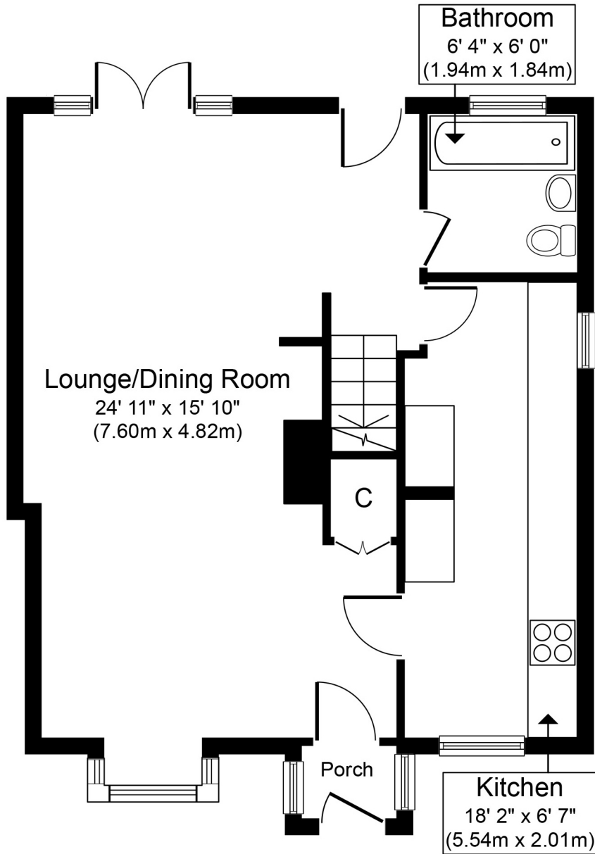
Ground Floor Approximate Floor Area 565 sq. ft. (52.5 sq. m.)
